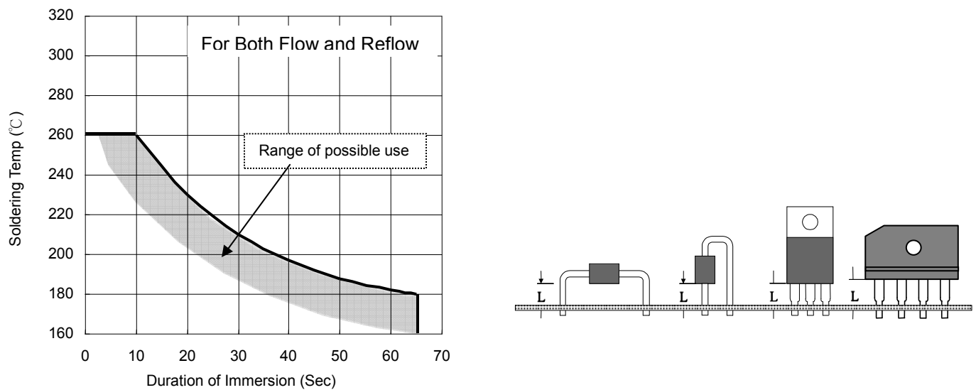
Figure 2. Rated Duration of Immersion vs. Solder Temperature
