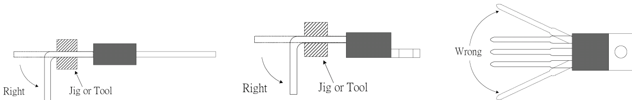
Figure 1. Bending Terminal Leads
